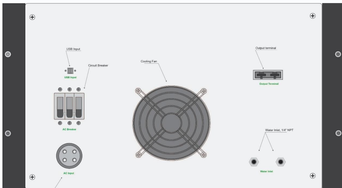
(Rear Panel)
